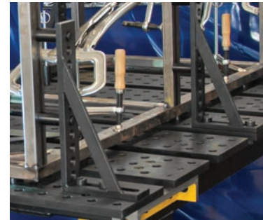
Insert V-Blocks to support round stock.
